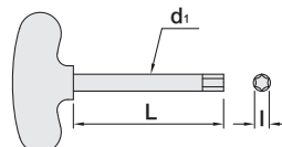
Fig.2 Allen wrench
