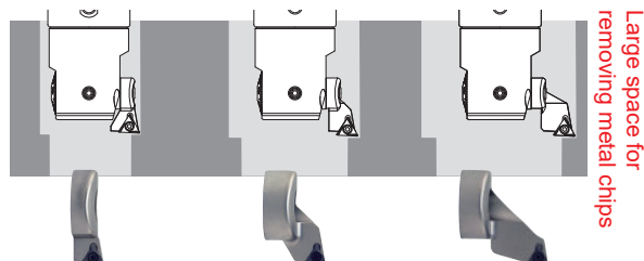
Insert seat SIC-1 Insert seat SIC-2 Insert seat SIC-3
